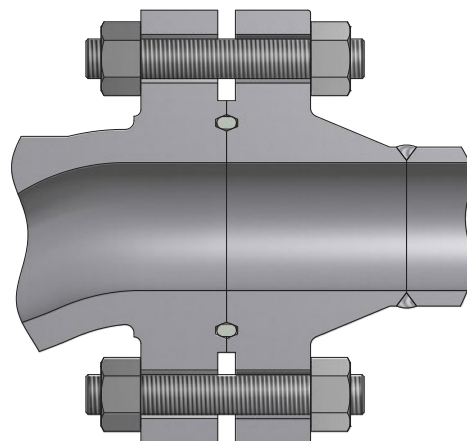
BRIDA RTJ (FIGURA 7)
